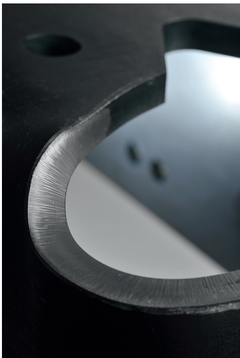
Trailer part made of 12 mm Armstrong® Ultra 700MC, laser cut and bent
